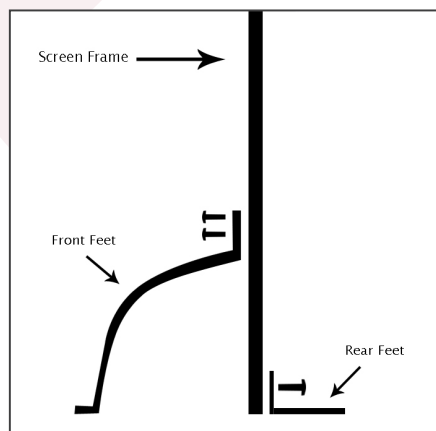
Assembly Profile
